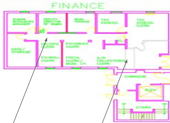
FIRST FLOOR PLAN 1/78-21-0 NOTE: ENTIRE BUILDING HAS NOT BEEN FIELD MEASURED
